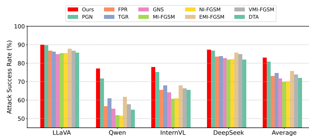
Figure 6: Attack Success Rate on LLaVA-v1.5-7B, Qwen 2.5-VL-7B-Instruct, InternVL 2.5-8B and DeepSeek-VL-7B-Chat. The adversarial examples are generated on ViT-B/16.
