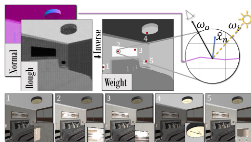
Figure 3: Importance-based Light Sampling. We render RGB images (bottom) from our generated PBR maps and a sampled light source as input (top). We employ multinomial importance sampling based using the inverse roughness to select less rough pixels more often (red squares). The light direction is then the viewing direction to the pixel reflected by its normal. The rendered images thus contain more specular effects, which provides better gradients during training.
