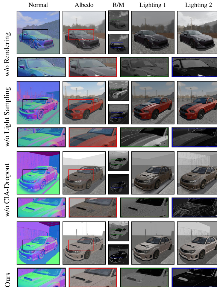
Figure 12: Additional ablations. We compare our full method against ablations that do not use the rendering loss (w/o Rendering), use uniform light sampling instead of importance-based light sampling (w/o Light Sampling), and do not use dropout in the cross-intrinsic attention (w/o CIA-Dropout). Without the rendering loss (Section 3.2.2), the PBR maps lose their semantic meaning, e.g., there are baked-in shadows in the albedo and the generated images appear “averaged out”. Importance-based light sampling (Section 3.2.2) and CIA dropout (Section 3.2.1) both increase the sharpness of individual PBR maps, e.g., the roughness/metallic images have realistic details without baked-in textures. Overall, all components improve the quality of rendered images under varied lighting conditions.
