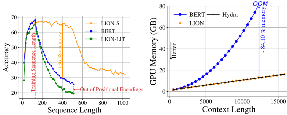
Figure 9: (Left) MLM Acc. for different sequence lengths. LION-S is able to generalize to larger sequence lengths and does not require positional encodings. (Right) GPU Memory for different sequence lengths. Results for the LARGE (334M) scale. The memory employed by LION and Hydra scales linearly with the sequence length, being able to process a sequence length of \sim 16,000 tokens with less than 20GB. Contrarily, the memory employed by BERT scales quadratically, going out of memory (80GB) at a sequence length of \sim 12,000 tokens.
