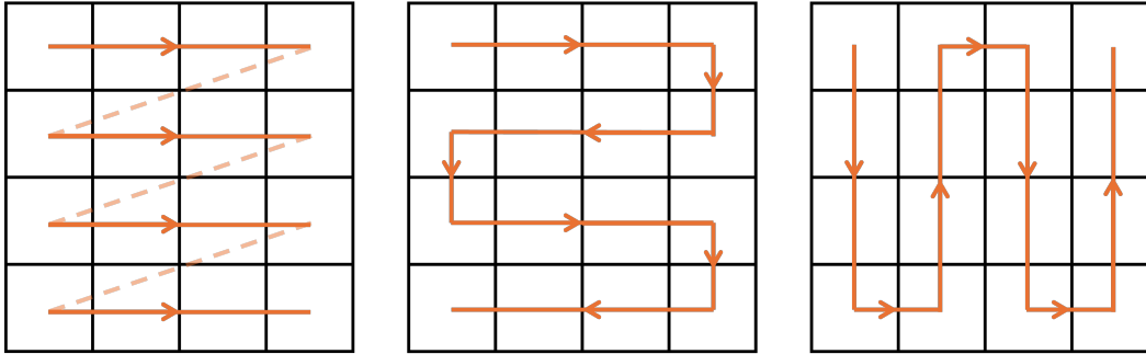
Figure 11: Reordering of patches . Left is the naive approach to flatten images, also used in LION-S. Center and right figures are the new approaches applied in LION-S ‡ to consider further spatial information.
