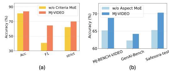
Figure 4: (a): Compare MJ-VIDEO with “w/o Criteria MoE”, where average results of Acc, F1, and strict metrics are evaluated over 5 aspects; (b) Compare MJ-VIDEO with “w/o Aspect MoE” on MJ-BENCH-VIDEO, Safesora-test and GenAI-Bench.
