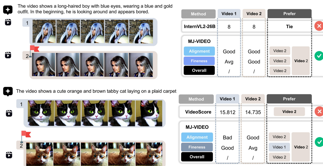
Figure 8: More cases of video reward modeling with MJ-VIDEO and other baselines.
