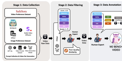
Figure 2: Three-stage curation process of MJ-BENCH-VIDEO.
