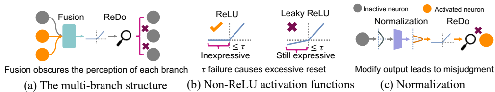
Figure 2: Key techniques involved in advanced models may reduce the efficiency of activation-based metrics. (a) The final activation values observed after branch fusion no longer accurately reflect the individual contributions of neurons in each branch. (b) A near-zero value fails to represent the expressivity with non-ReLU activation function. (c) Normalization confuses ReDo by modifying the neuron's outlier output.
