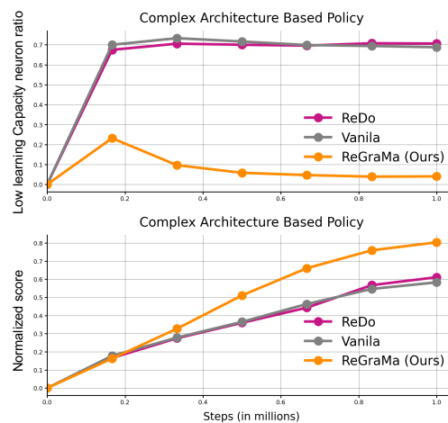
Figure 1: Dormant neuron metric struggles in advanced vision RL BRO-net agent [Nauman et al., 2024b]. Neuron resetting based on the dormant neuron index (ReDo) cannot restore the learning capacity of the agent, which limits its effectiveness. The curves record normalized score across 3 image-input tasks (15 runs per method), i.e., Dog Stand, Dog Walk, Dog Run.
