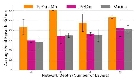
Figure 9: ReGraMa is more robust under network scaling. Results averaged over four DMC tasks with 12 seeds per method.
