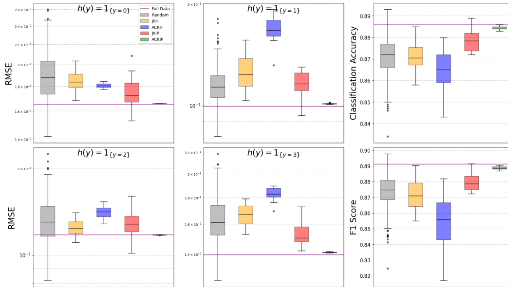
Figure 24: Results for Imbalanced dataset for compressed sets of size m = 250 . The RMSE across a variety of test functions is reported, with the IQR highlighted for each method. Outliers are calculated as being above Q_3 + 1.5\text{IQR} and below Q_1 - 1.5\text{IQR} .
