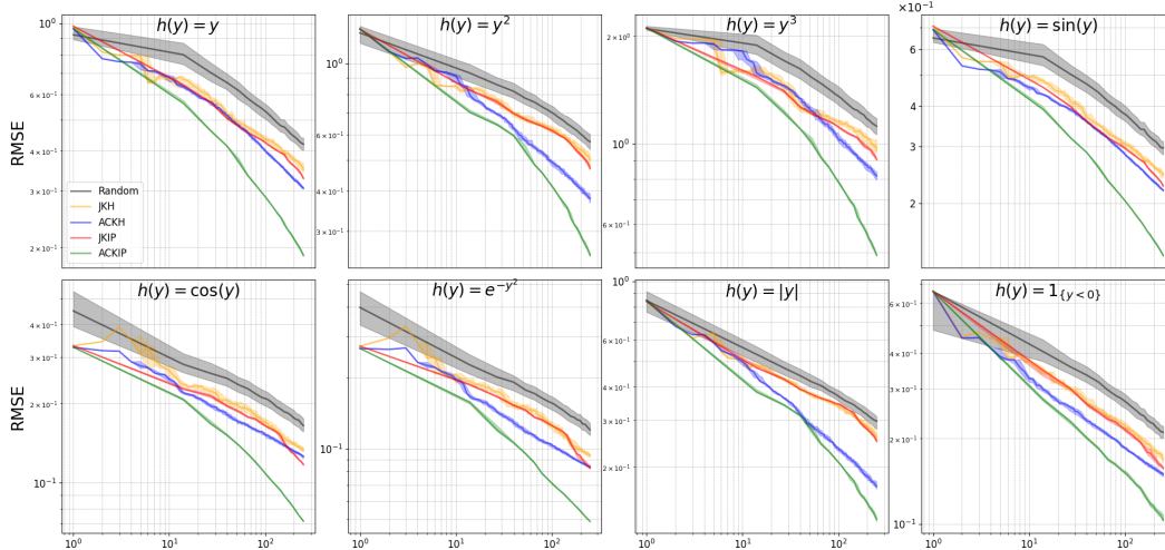
Figure 14: Results for the Superconductivity dataset; the RMSE is calculated against the full data estimates of \mathbb{E}[h(Y) \mid X = x_i] as the true values are not available. The RMSE is reported across a variety of test functions, as the size of the compressed set increases. For JKH (orange), JKIP (red), ACKH (blue), and ACKIP (green), we display the median performance (bold line) with the 25th-75th percentiles (shaded region) over 20 runs. The error of random sampling (black) over 500 runs is also plotted for comparison.
