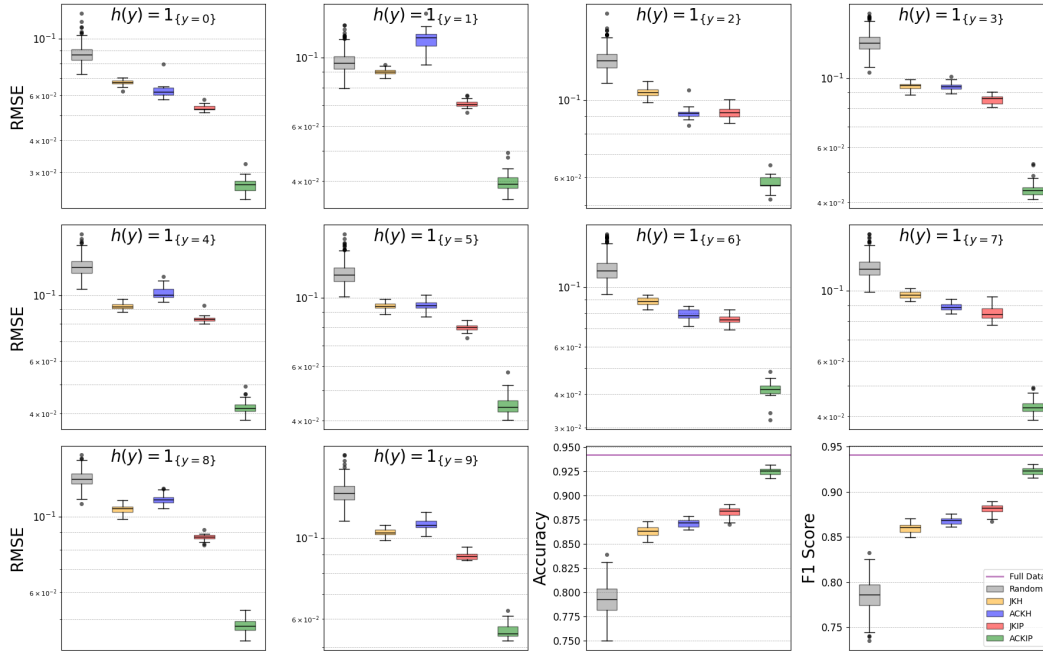
Figure 30: Results for MNIST data for compressed sets of size m = 250 ; the RMSE is calculated against the full data estimates of \mathbb{E}[h(Y) | X = x_i] as the true values are not available. The RMSE across a variety of test functions is reported, with the IQR highlighted for each method. Outliers are calculated as being above Q_3 + 1.5\text{IQR} and below Q_1 - 1.5\text{IQR} .
