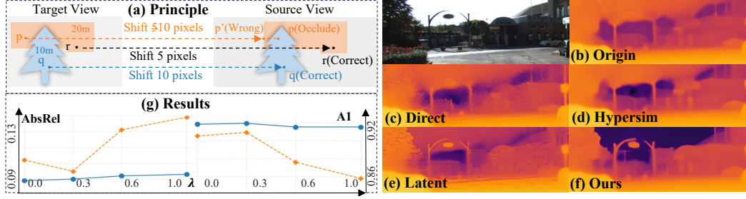
Figure 3: The attempts to preserve the SD prior. The meanings of (a)-(f) are detailed in Sec. 3.2. Notably, while (e) demonstrates superior visual quality, it erroneously interprets surface textures (e.g., house windows) as depth edges. (g) shows the performance variations under different \lambda settings for photometric supervision (Eq. 5) and latent supervision (Eq. 4). The complete metrics and their definitions are provided in Sec. E.4.
