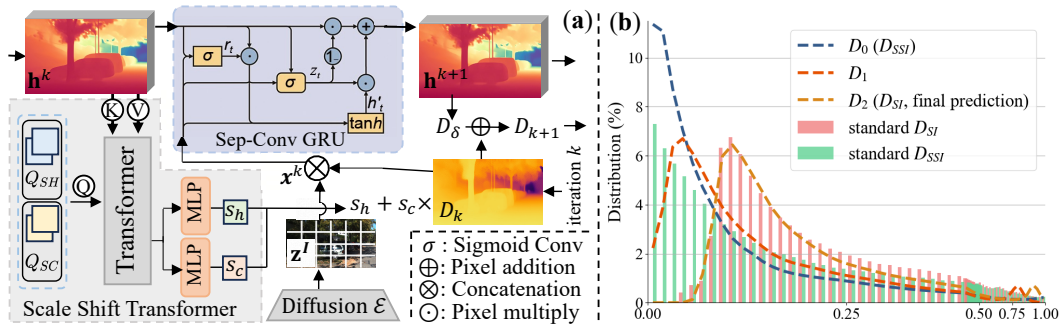
Figure 4: (a): Model Structure of SSG. It corresponds to the gray rectangle shown in Fig. 2, standing for an iteration within two consecutive ones. The pipeline of SSG is comprehensively described in Sec. 3.3 (DepthHead is omit in (a) for clear). (b): Depth distribution alignment visualization. We statistically analyze each stage of Jasmine’s SSG module on the KITTI test set. The standard SI and SSI depths are obtained by applying Eq. 9 and dividing the maximum value to the depth GT, respectively.
