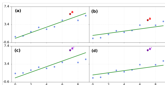
Figure 6: Comparison of different de-normalization schemes. The blue points are predictions after alignment and the green line is the ideal GT depth. Sub-figures (a,c) are the results of LSQ alignment, while (b,d) are median alignment.
