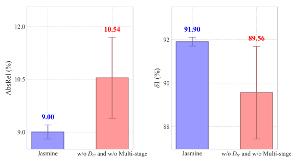
Figure 9: Error Bar Analysis on KITTI Eigen test split. We conduct this analysis through multiple training runs and observe the performance oscillations after 25k steps.
