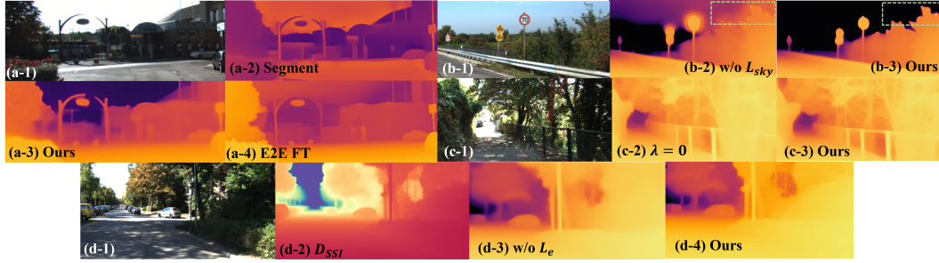
Figure 7: Qualitative Ablation Study of Adaptive Loss. Notably, while (a-2) demonstrates superior visual quality, it exhibits an entirely inaccurate depth distribution. (a-4) is the result of E2E FT, which can serve as a pseudo-label here.
