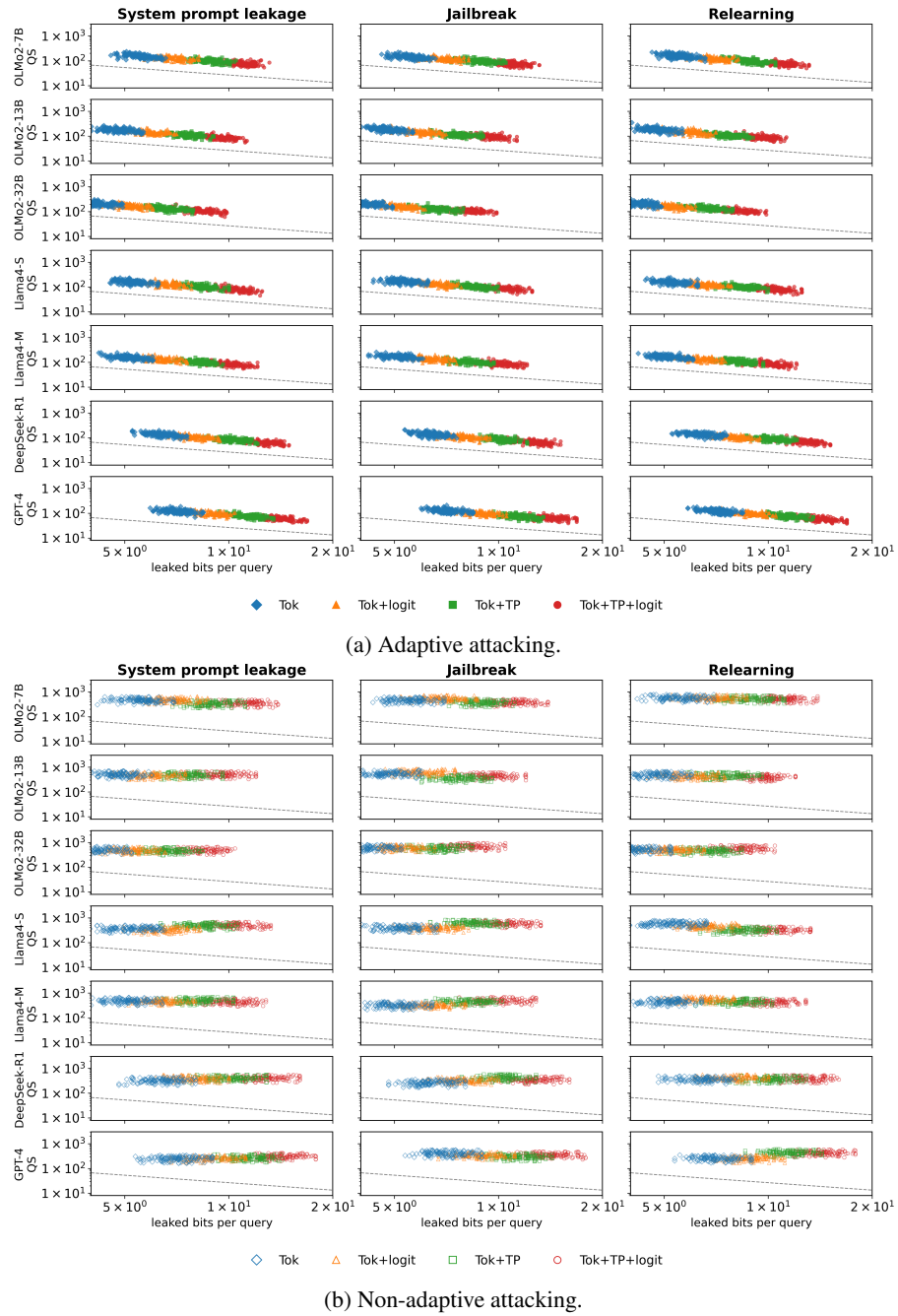
Figure 1: Measured number of queries to success N ( y axis, \log_{10} scale) required to reach a success probability 1 - \varepsilon versus the single-query mutual information I(Z; T) (horizontal axis, \log_{10} scale). Columns correspond to the three attack tasks: system-prompt, jailbreak, and relearning attacks, while rows list the seven target LLMs. Marker shapes and colors denote the leakage signals available to the adversary. The dashed black line shows the information-theoretic lower bound N_{\min} .
