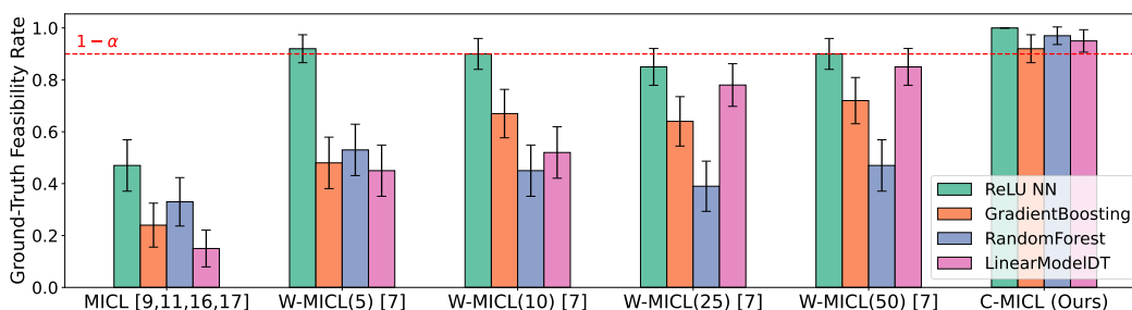
Figure 1: Empirical ground-truth feasibility rate of optimal solution across MICL methods on 100 optimization problem instances. Our Conformal MICL approach (rightmost bars) consistently achieves the target ground-truth feasibility rate \geq 90\% regardless of the underlying base model used. Previous methods demonstrate variable performance below this theoretical guarantee. Error bars correspond to 95% confidence intervals for ground-truth feasibility rates across 100 runs.
