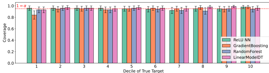
Figure 15: Empirical out-of-sample coverage at \alpha = 5\% for all predictive models, evaluated on 1,000 test points and stratified by deciles of the true output y . Our conformal prediction sets achieve the desired coverage level across deciles. Notably, the ground-truth feasibility threshold ( y \geq 50 ) lies in the 9th and 10th deciles, where all methods achieve valid empirical coverage, providing empirical support for the assumptions in Theorem 4.1.
