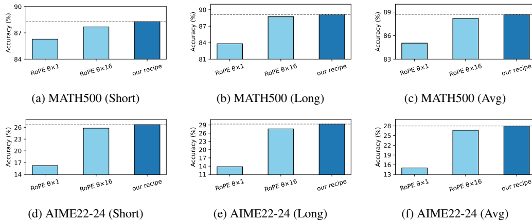
Figure 11: Comparison of reasoning accuracy across different configurations. Results are reported on MATH500 (top row) and AIME22-24 (bottom row), with separate evaluation for short, long, and average context cases. Our proposed recipe (dark blue bar, dashed line) consistently outperforms the baseline RoPE \theta \times 1 and the extended-context baseline RoPE \theta \times 16 , demonstrating that enhancing long-context capability prior to reasoning fine-tuning yields stable and significant accuracy improvements, enhancing models' reasoning ability.
