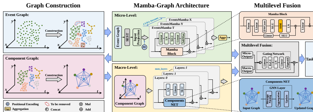
Figure 1: The overall workflow of EventMG comprises three main modules: 1) Graph Construction , which constructs the micro-level Event Graph and macro-level Component Graph; 2) Mamba-Graph Architecture , which performs spatiotemporal modeling at both levels; and 3) Multilevel Fusion , which integrates outputs across levels to produce the final spatiotemporal representation for downstream tasks.
