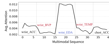
Figure 9: Averaged Attention map for a batch across the multimodal sequence.
