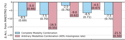
Figure 6: Ablation of MAESTRO: absolute accuracy drop ( \Delta ) from full model, with ablated scores in parentheses.
