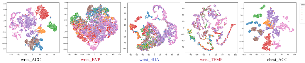
Figure 17: t-SNE projections of the unimodal models’ latent representations for each modality in DaliaHAR (supporting results for Table 5 in Section 4.2 in the main paper).
