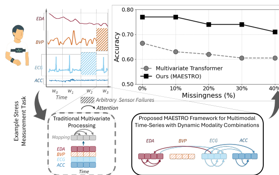
Figure 1: Illustration of traditional multivariate processing vs. our multimodal handling of sensor data, highlighting our method's superior performance and robustness.
