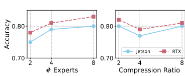
Figure 7: Sensitivity Analysis.
