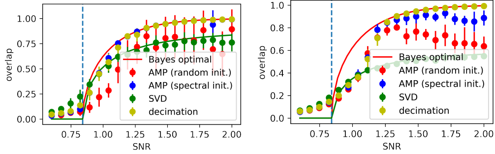
Figure 6: The performance of AMP and decimation AMP. Left: r = k = 2 . Right: r = k = 10 .
