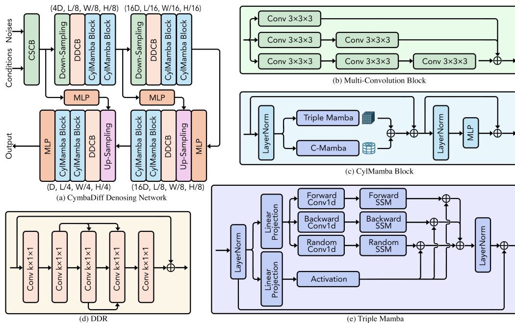
Figure 3: Architecture of the CymbaDiff denoising network. CylMamba denotes cylinder mamba block. Refer to the text for details.
