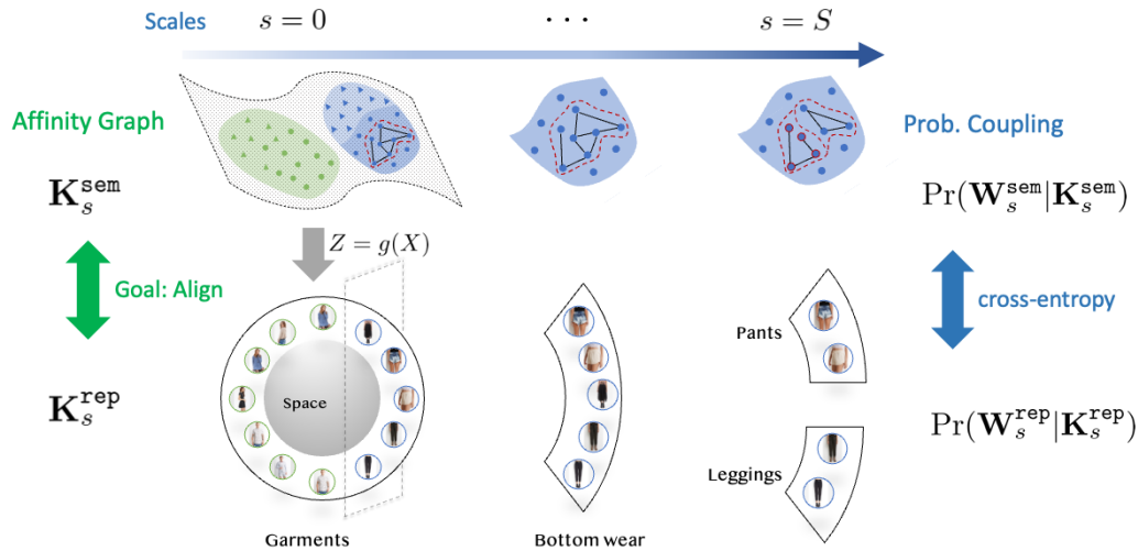
Figure 1: Illustration of multi-level contrastive learning. An ideal scenario where the learned representations exhibit a hierarchical structure that captures both broad categorical distinctions and fine-grained semantic relationships. Our approach identifies and optimizes local worst-case regions (highlighted in red) where representation affinity deviates significantly from the semantic affinity. Here, the affinity matrices K_s^{\text{sem}} and K_s^{\text{rep}} represent pairwise semantic and representation relationships, respectively, as defined in (3) and (4).
