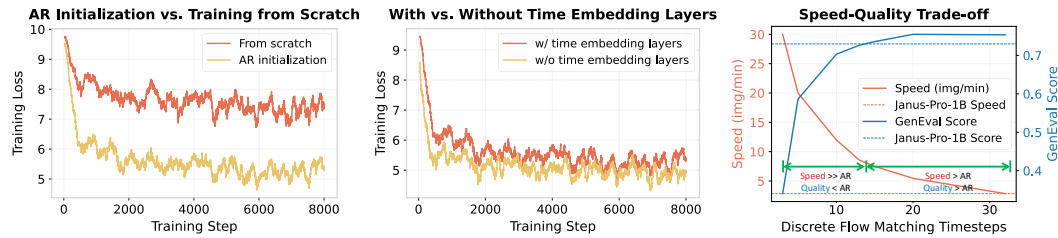
Figure 5: Comparison of training loss and speed-quality trade-off. (Left, Middle) AR initialization and removing time embedding layers both reduce training loss. (Right) With fewer timesteps, FUDOKI achieves much higher speed but slightly lower quality than AR; at the optimal timestep, both metrics surpass the AR.
