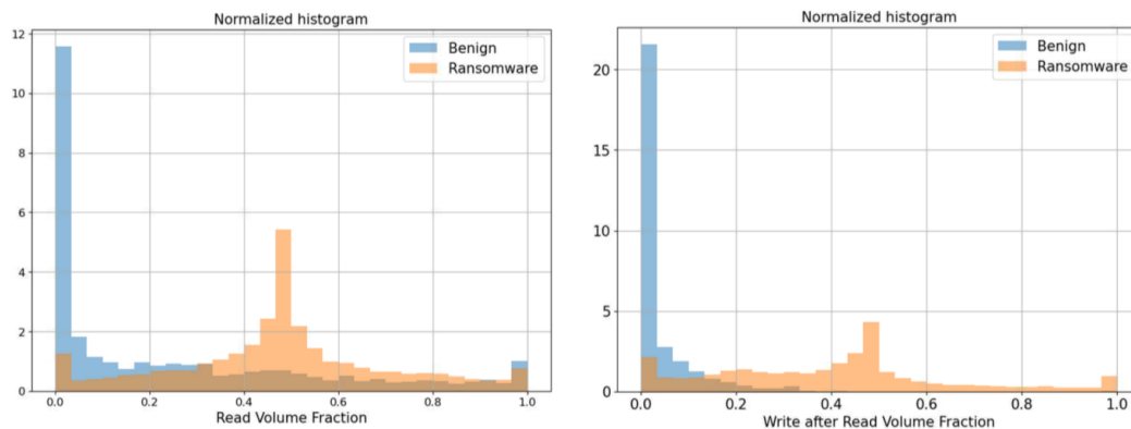
Figure 1: Normalized histograms for the \text{frac}_R and \text{frac}_{WAR} across 5,809 benign chunks and 21,243 ransomware chunks. All chunks have the same traffic volume equal to 0.5GiB.
