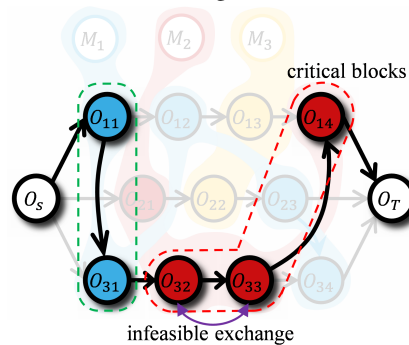
Figure 5 Infeasible exchange caused by the N5 neighborhood in FJSP. Dotted lines of different colors are critical blocks.
