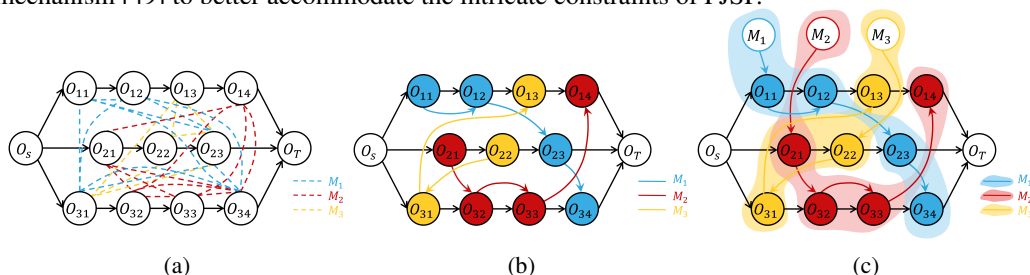
Figure 1 Graph representations of FJSP. (a) FJSP instance in a disjunctive graph; (b) feasible solution in a disjunctive graph; (c) feasible solution in our graph.
