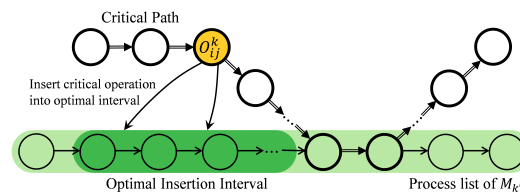
Figure 2 Nopt2 neighborhood structure.
