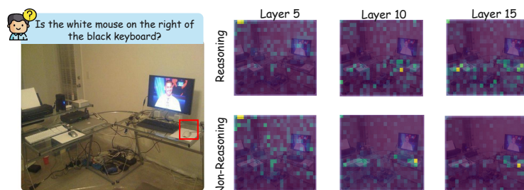
Figure 10: Case Study 2: Attention Heatmap in Object Localization.
