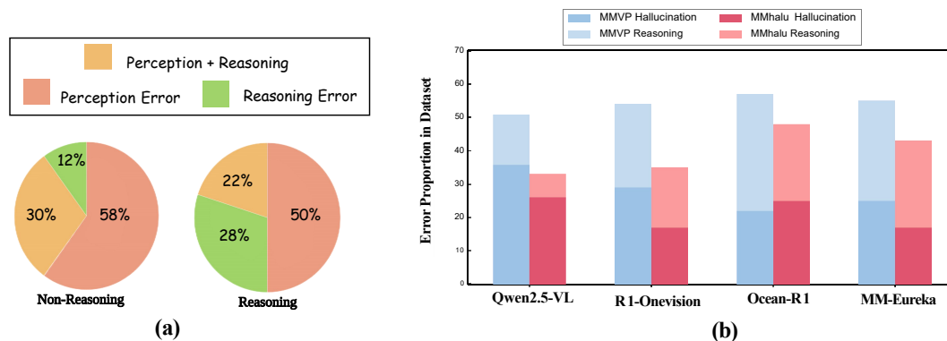
Figure 12: Error type distribution and error proportions across reasoning and non-reasoning models in Bingo benchmark. (a) Pie charts showing the distribution of perception and reasoning errors for non-reasoning and reasoning models, with the breakdown of perception error, reasoning error, and combined perception & reasoning errors. (b) Bar chart illustrating error proportions in the MMVP and MMhalu benchmarks, comparing hallucination and reasoning errors across reasoning models.
