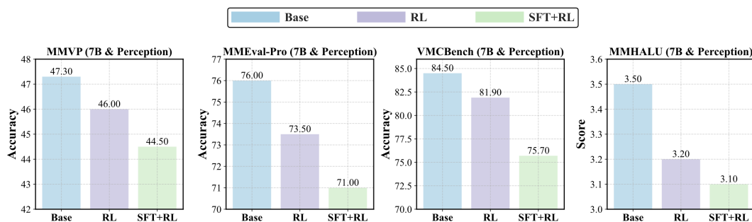
Figure 3: Performance across four perception benchmarks comparing Base, RL, and SFT+RL.
