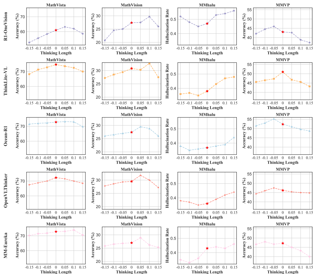
Figure 13: Model performance variation of the Latent State Steering strategy. The star symbol represents the original thinking length of the model without steering or test-time intervention.
