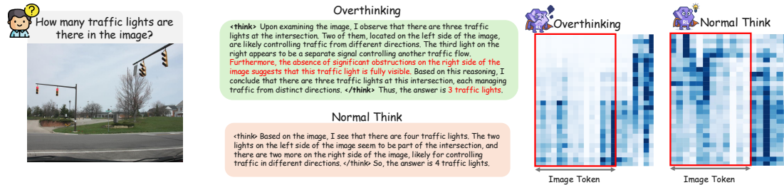
Figure 11: Attention shift in the reasoning model under different reasoning length.
