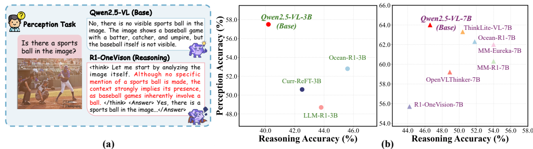
Figure 1: (a) Example of outputs from a reasoning model and a non-reasoning model on a perception task. Red highlights indicate visual hallucination. Multimodal reasoning models are generally more prone to amplifying hallucinations during the reasoning process compared to their non-reasoning counterparts. (b) Performance of different models on reasoning and perception tasks in the RH-Bench dataset. Better performing models are positioned in the upper right corner. Baseline non-reasoning models of varying scales typically exhibit weaker reasoning capabilities and fewer hallucination, whereas reasoning models display the opposite trend.
