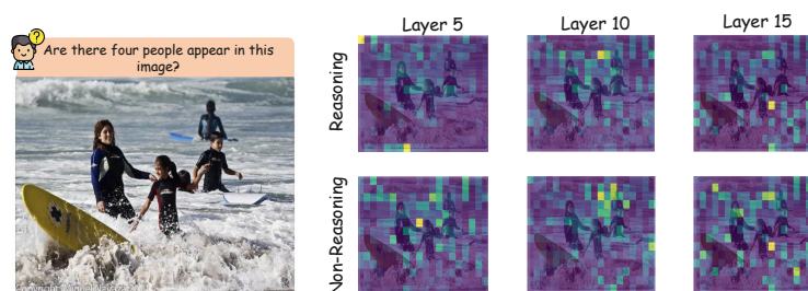
Figure 9: Case Study 1: Attention Heatmap in Counting Tasks.
