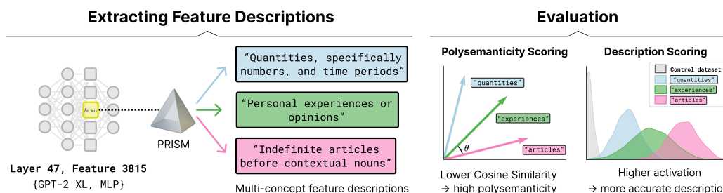
Figure 1: Overview of the PRISM framework. PRISM captures multiple concepts per feature, enabling the detection of both polysemantic and monosemantic features, unlike prior approaches that constrain each feature to a single description. For example, feature 3815 in layer 47 was previously labeled as monosemantic [20], whereas PRISM reveals that it responds to multiple distinct concepts. Polysemanticity scoring summarizes how diverse the concepts associated with a feature are, while description scoring assesses how well each concept aligns with the feature’s activation distribution.
