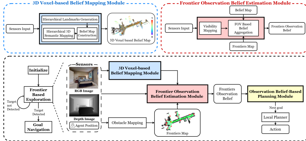
Figure 2: BeliefMapNav pipeline: The agent initializes with a 360° rotation. During exploration, the 3D voxel-based belief mapping module fuses sensor input, the 3D hierarchical semantic map, and landmarks to create a belief map. The frontier observation belief estimation module computes frontier observation belief from the belief, frontiers, and visibility maps via FOV-based aggregation. The observation belief-based planning module selects the next goal based on this belief and outputs navigation actions. Upon detecting the target, the agent navigates to it.
