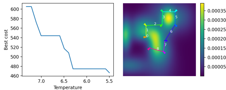
Figure 7: Result demo of the algorithm. The chart on the left shows the relationship between the cost and the temperature under a run. The chart on the right shows the path generated by the algorithm. The number on the lines indicates the order of visiting the frontiers. The arrow at each frontier is the orientation. The color of the background represents the distribution of the occurrence probability. The observation probability of a frontier is the sum of the weights of all points within a sector in front of the frontier, representing points within the FOV of the robot.
