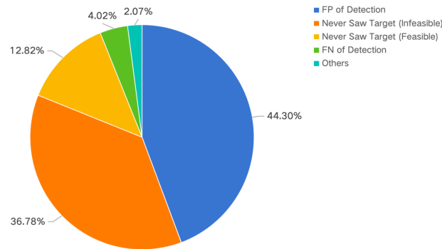
Figure 8: The proportion of different causes of failure in the HM3D dataset.
