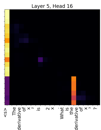
(a) Attention probabilities at layer 5, head 16.
