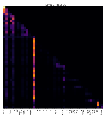
(a) Attention probabilities at layer 3, head 30.
