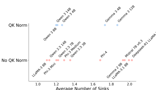
Figure 6: Sink Count in Models with QK Norm. For each model, the average number of sinks is computed across all attention heads and layers.
