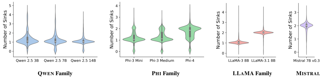
(a) Attention Sink Counts. Counts are computed for each head using Equation 1, and their distribution is visualized for each model using violin plots.
