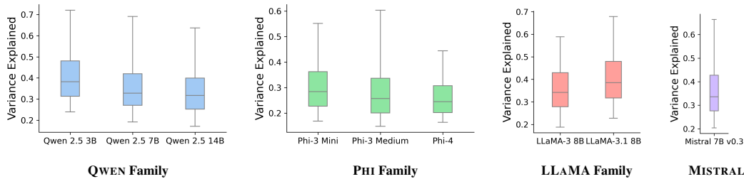
(b) Variance Explained by Tags. The metric is computed for each head using Equation 2, and summary statistics are shown for each model using box plots. Boxes indicate the 25th, 50th, and 75th percentiles, while whiskers represent the 5th and 95th percentiles.
