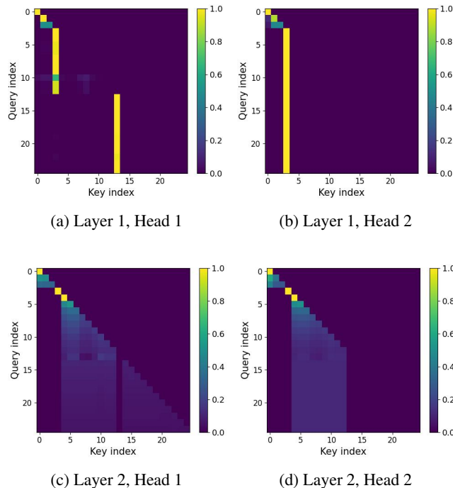
Figure 18: Attention probability maps for each head and layer. Each attention head is dedicated to solving a specific portion of the task, which in the first layer, requires the different attention heads to form distinct sinks and tags that the model uses constructively to create the desired probability distributions in the second layer.
