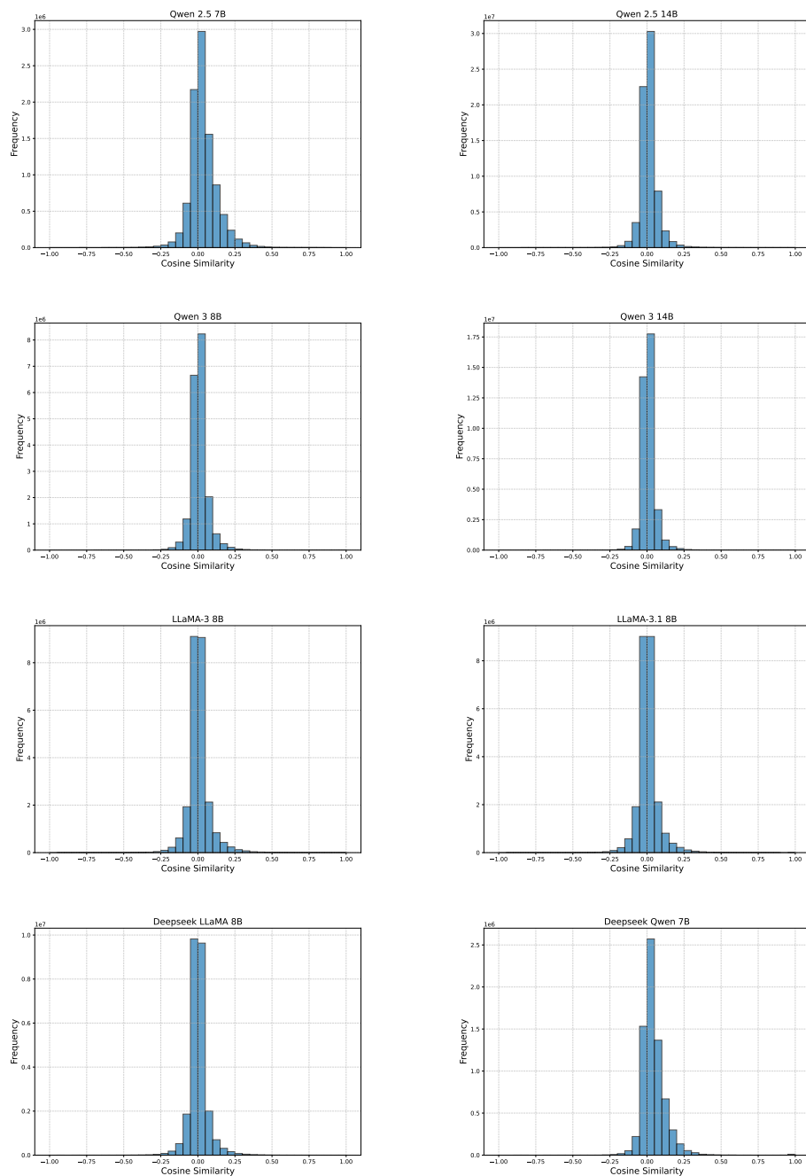
Figure 19: Cosine Similarity Between Tags. Histograms of the cosine similarity between distinct tags across all layers and heads. The tags typically exhibit very small cosine similarity implying that they are close to orthogonal and do not interfere with one another.
