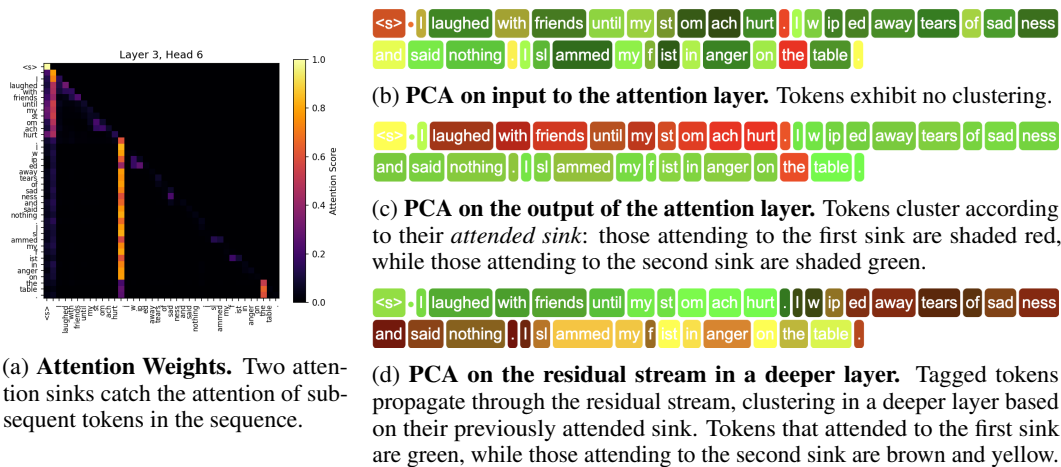
Figure 2: Qualitative analysis of the ‘catch, tag, release’ mechanism. The second and third subplots use PCA-based coloring of embeddings, described in Section 2. Appendix A presents additional measurements across a wide range of models, layers, attention heads, and prompts, including chain-of-thought [Wei et al., 2022], and zero-shot chain-of-thought [Brown et al., 2020].
