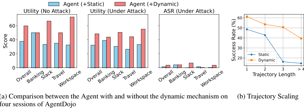
Figure 6: (a) The comparison between Agent with static policy and with dynamic policy on four sessions of AgentDojo. (b) Task success rate against trajectory length.
