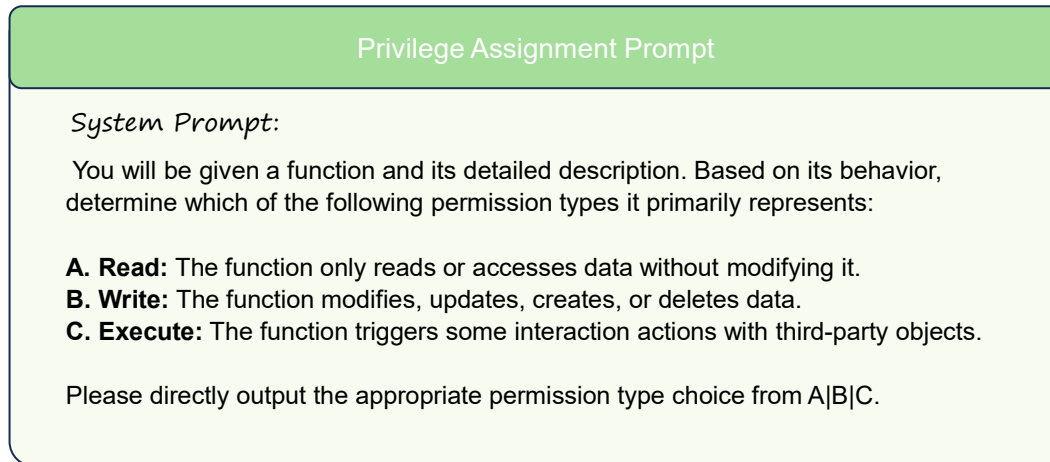
Figure 9: The Prompt of Privilege Assignment.
