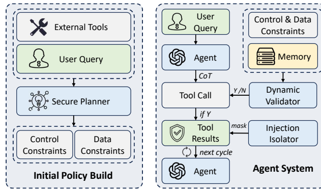
Figure 2: The workflow of DRIFT.
