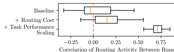
Figure 2: Models trained with routing cost and task-based scaling exhibit more stable routing. Correlations are calculated between the routing patterns across 20 training runs of each model setup.
