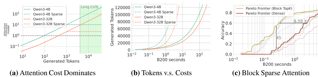
Figure 2: (a) Inference cost is dominated by attention, which is 100 \sim 1000\times more than model parameter computation, sparse attention fundamentally mitigates this bottleneck. (b) Under the same resource constraint, sparse attention can generate massive tokens out of the reach of dense models, which is proven to enhance the effectiveness of test-time scaling. (c) Simple block sparse attention yields substantial gains—improving accuracy by 45 points in the low-cost regime and achieving equivalent accuracy while using 8.58\times fewer resources.
