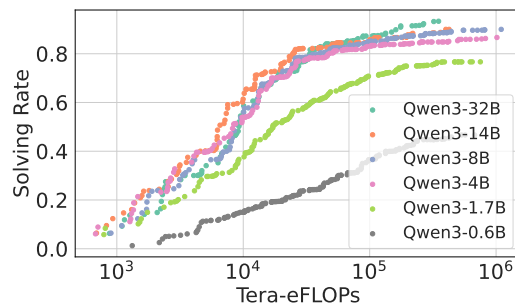
Figure 13: AIME Pareto Frontier (Best-of-N) with Max Cost Models. We re-plot Figure 6a using max cost models. The Pareto Frontier is very similar under different cost models.
