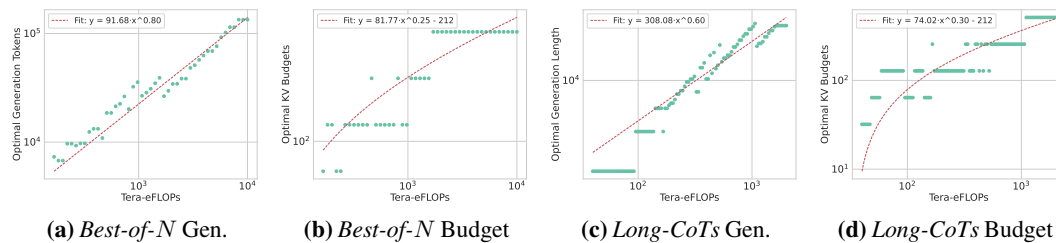
Figure 9: Tradeoff Between Generated Tokens and KV Budget. We empirically investigate how to balance the tradeoff between generating more tokens and allocating a larger KV cache budget, which may yield more accurate but potentially shorter outputs. Using Qwen3-8B as a representative model, we fit curves to characterize this tradeoff. For Best-of-N , we find that for every doubling of the total compute cost, the optimal KV budget increases by a factor of 1.18\times , while the total number of generated tokens increases by 1.74\times . For Long-CoT , the corresponding factors are 1.23\times and 1.52\times , respectively. Notably, when the KV budget is small, the computational cost is dominated by model parameter-related computation rather than token generation or KV cache usage. We incorporate a model-specific constant into the cost model to account for this effect.
