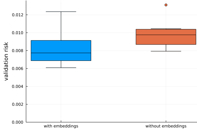
Figure 3: Validation risks of GBT_{f,1,x,0} (with embeddings, on the left) and GBT_{f,1,I_N,0} (without embeddings, on the right), estimated using 10-fold cross validation. The box plots report the minimum, 1st quartile, median, 3rd quartile and maximum. Outliers are also shown.
