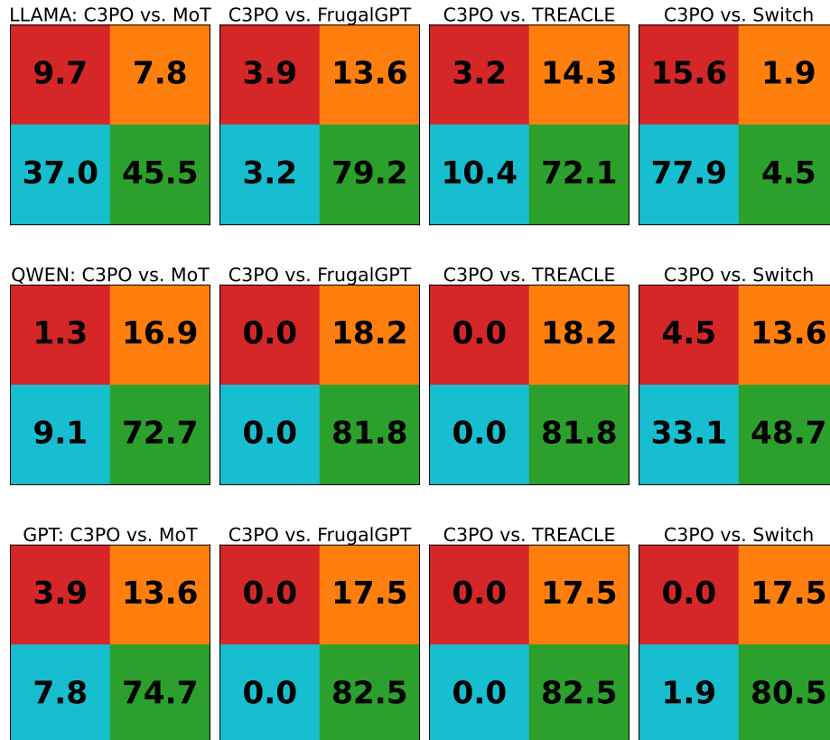
Figure 15: Percentage of 'very bad', 'bad', 'good', and 'very good' questions for each baseline and LLM cascade from the AQuA dataset
