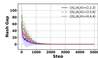
Figure 1: Nash gap
