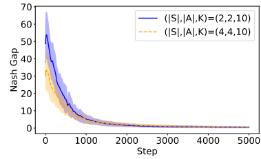
Figure 7: Nash gap for ARAM
