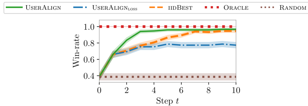
(b) Win-rate w.r.t. increasing steps
