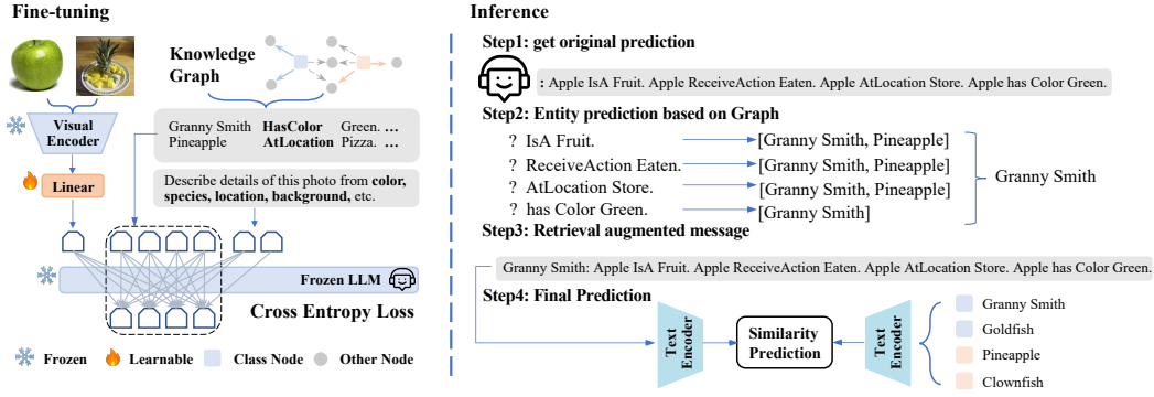
Figure 2: Left: In knowledge graph-enhanced learning, image embedding, knowledge-enhanced ground-truth embedding, and question embedding are input to Frozen LLM to generate predicted embedding; cross-entropy loss updates the linear layer. Right: In knowledge graph-augmented inference, relations from predicted text are extracted to create graph-augmented text, producing the final prediction.
