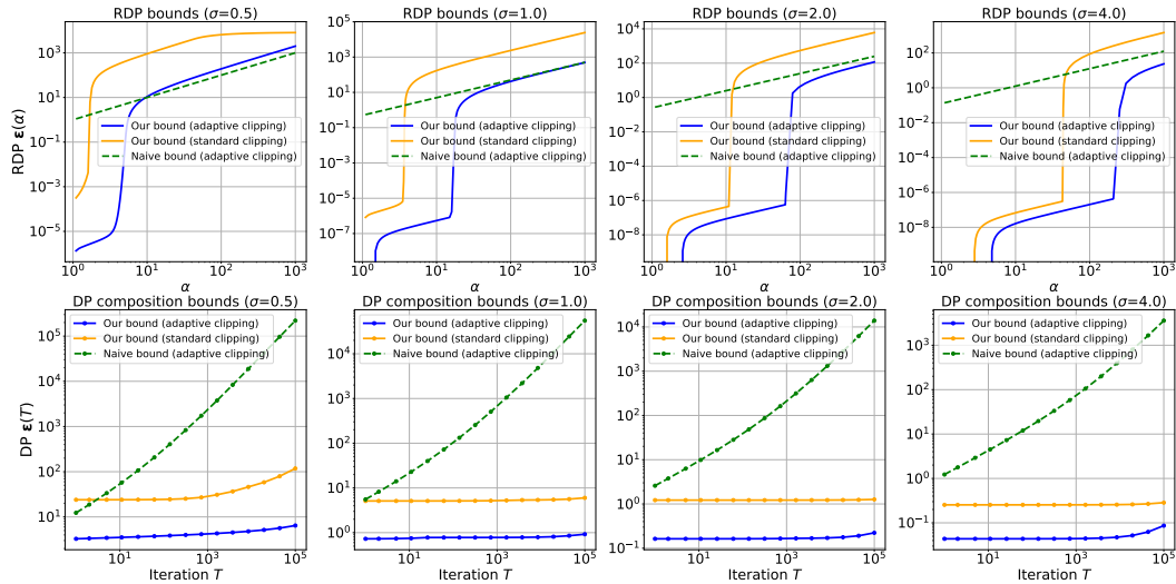
Figure 5: Comparison of per-iteration RDP bound \varepsilon(\alpha) (first row) and DP composition bound \varepsilon_{\text{DP}}(T) over T iterations (second figures), under different noise level \sigma . Our bound (adaptive clipping) refers to the bound in Theorem 4.1. Our bound (standard clipping) refers to the similar amplification bound with standard clipping in place of adaptive clipping. Naive bound is simply the Gaussian mechanism RDP bound \varepsilon(\alpha) = \alpha/\sigma^2 .
