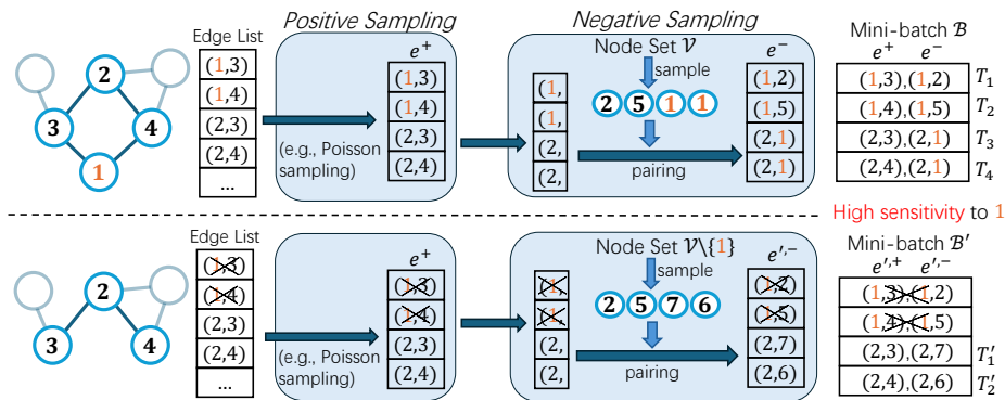
Figure 1: The mini-batch sampling process in relational learning is a two-stage sampling that first samples edges from full edge list (positive sampling) and then construct negative edges based on the sampled positive edges (negative sampling). A node can occur in multiple positive and negative edges, leading to a high sensitivity. Note that the entire batch changes due to the removal of node 1.
