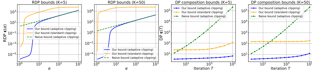
Figure 2: Comparison of per-iteration RDP bound \varepsilon(\alpha) (left two figures) and DP composition bound \varepsilon_{\text{DP}}(T) over T iterations (right two figures), under different capped node degree K . Our bound (adaptive clipping) refers bound Eq.(3). Our bound (standard clipping) uses similar amplification analysis but with standard clipping. Naive bound is the Gaussian RDP bound \varepsilon(\alpha) = \alpha/\sigma^2 .
