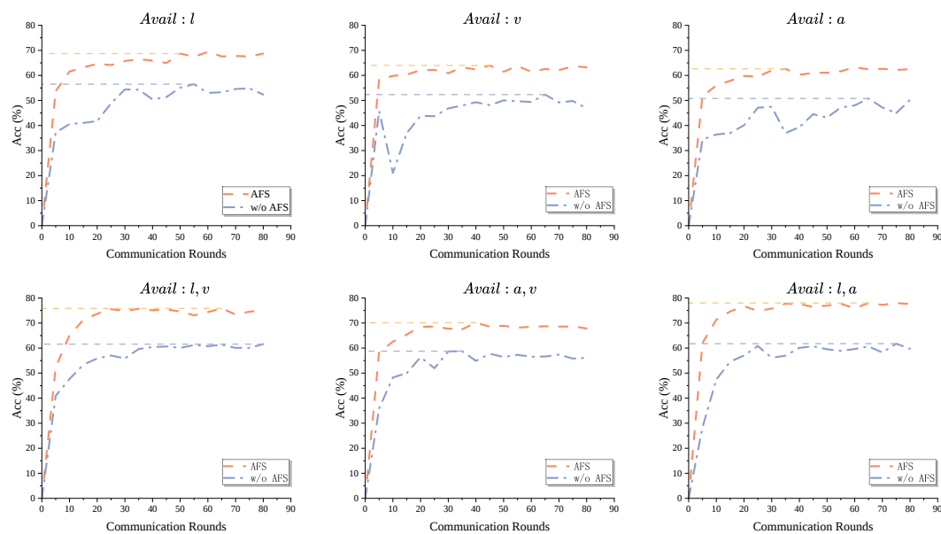
Figure 8: The ACC variation curves of models using AFS compared to models without AFS under all incomplete modality conditions.
