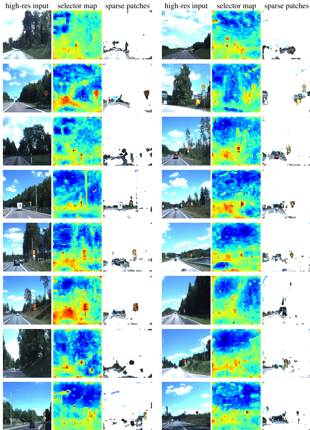
Figure 14: Adaptive Computation for Traffic Sign Recognition. We visualize the selector’s prediction of where to compute and the extractor’s sparse input for what to see. We do not finetune the selector; each pair shows different generalization scenarios, specifically for recognizing traffic signs on the Swedish Traffic Signs dataset [34].
