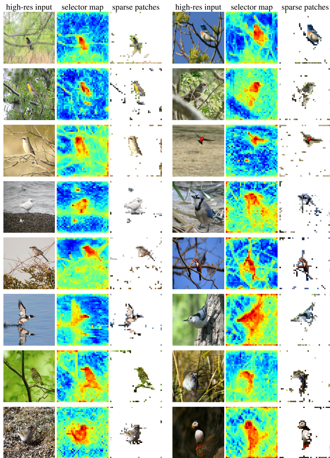
Figure 13: Adaptive Computation for Recognizing Birds. We visualize the selector’s prediction of where to compute and the extractor’s sparse input for what to see. We do not finetune the selector; each pair shows different generalization scenarios, specifically for bird recognition on CUB [41].
