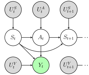
Figure 2: SCM of an LM agent with abstraction variable Y
