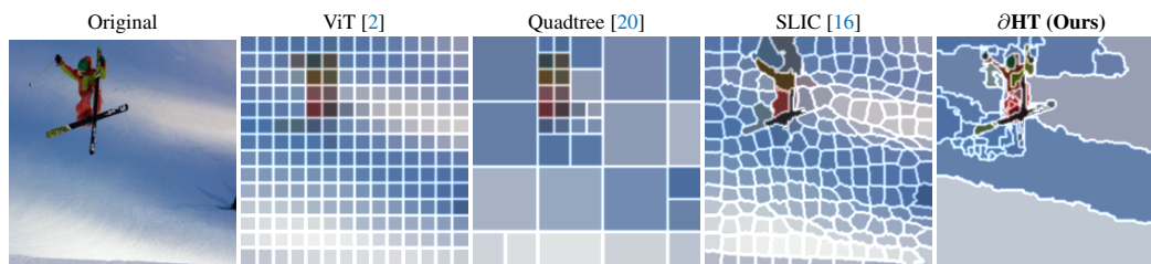
Figure 1: Comparing spatial granularity in visual tokenizers. \partial HT (right) provides an end-to-end learnable framework for multi-scale tokenization. We provide more examples in Figure E.6.
