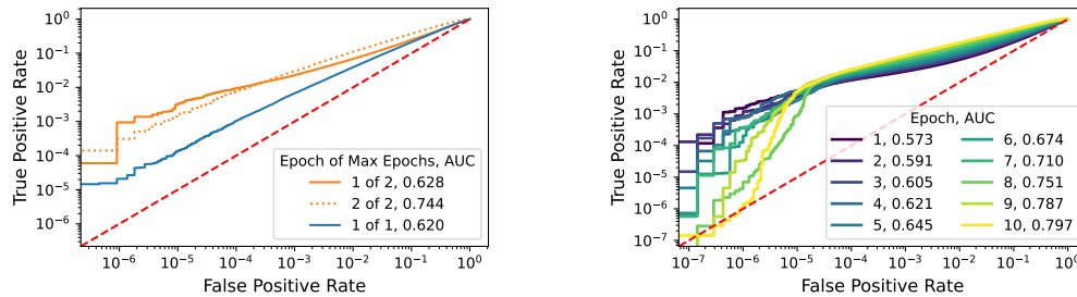
(a) 44M model, split dataset in half and train for 2 epochs, or train on the entire dataset for 1 epoch
