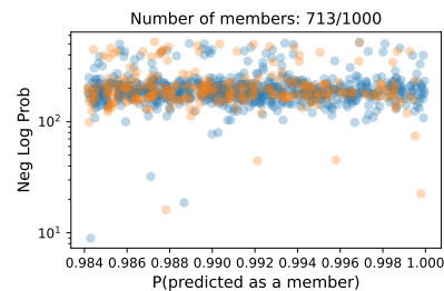
Figure 7: Extraction for 140M. Negative log-probability of the 50-token suffix (given the prior 50 tokens as prefix) for the 1,000 samples predicted most strongly as members.
