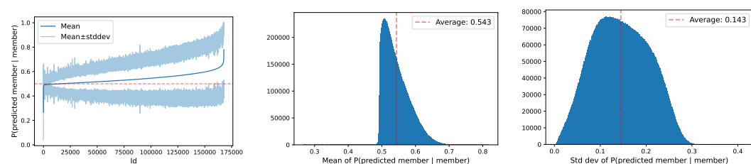
(a) Per-sample true positive probabilities (mean \pm standard deviation), ordered from smallest to largest. (b) Histogram of average per-sample true positive probabilities from Figure 21a. (c) Histogram of standard deviation of per-sample true positive probabilities from Figure 21b.
