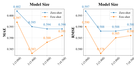
Figure 9: Model size analysis.
