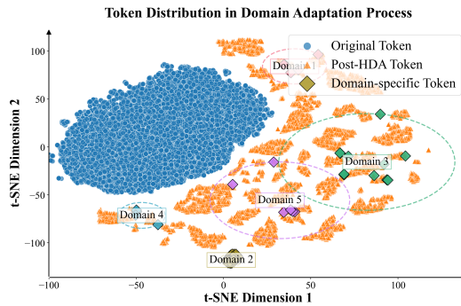
Figure 6: Domain adaptation visualization.
