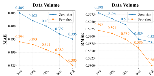
Figure 8: Pretraining data scaling analysis.
