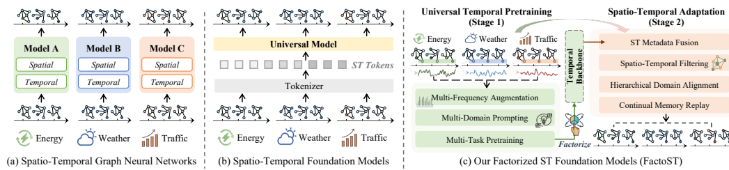
Figure 1: Evolution of ST modeling: (a) Traditional coupled STGNN design; (b) Joint ST pretraining in STFMs with tokens from different space and time; (c) FactoST's factorized paradigm.
