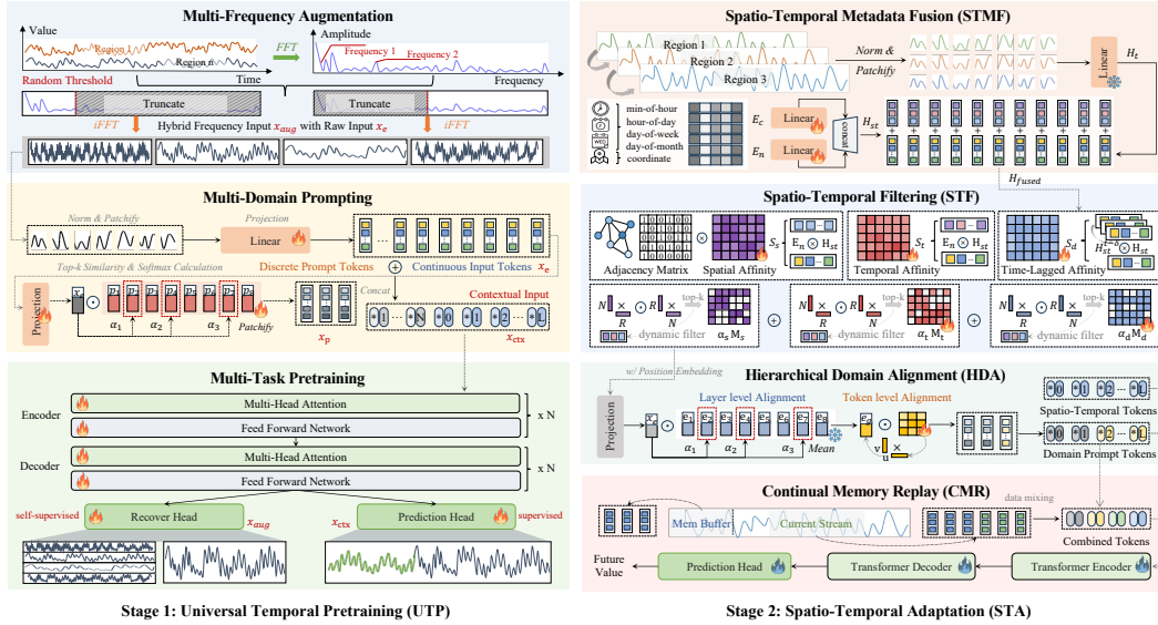
Figure 2: Overview of FactoST.
