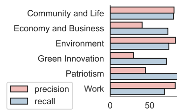
Figure 6: The precision and recall analysis for GPT-4.1 in YOUTUBE.
