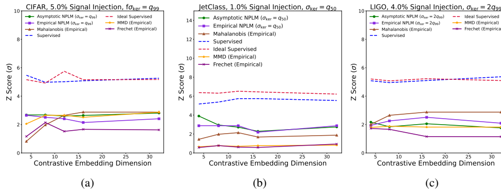
Figure 12: Z score as a function of embedding dimension for NPLM and baseline anomaly detection methods in the CIFAR-10 (a), JetClass (b), and LIGO (c) datasets. The best-performing kernel widths are chosen for presentation, and signal injection fractions are set such that NPLM has good but not fully-saturated sensitivity at the d = 4 baseline.
