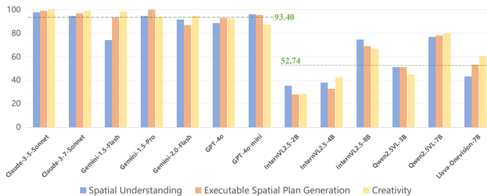
Figure 4: Bar chart of Output Success Rate (OSR) for MLLMs. Two green dotted lines indicate the average OSR of proprietary models and open-source models, respectively.
