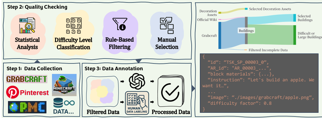
Figure 3: Data curation pipeline of MineAnyBuild . We conduct three core steps to curate our datasets: data collection, quality checking, and data annotation. On the right side, a Sankey diagram showing our data processing flow is presented, along with an example of simplified format of processed data.
