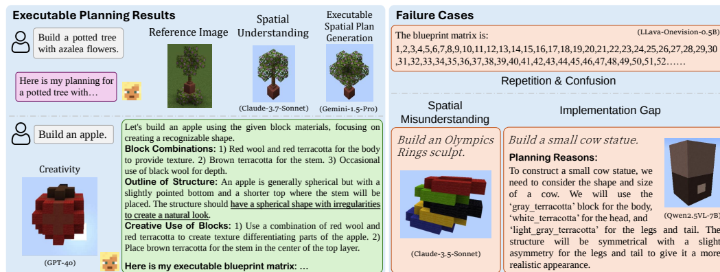
Figure 5: Visualization of executable planning results (left) and failure cases (right).
