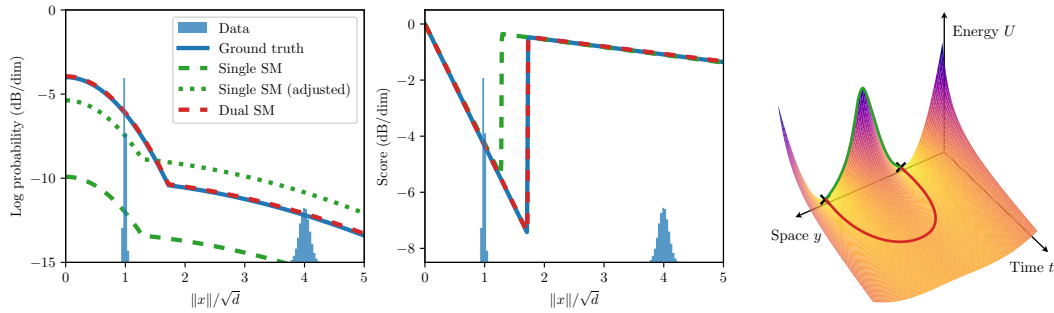
Figure 1: Comparison of single and dual score matching on recovering the energy of a scale mixture of two Gaussians in d = 1000 dimensions. Experimental details are provided in Appendix C.3. Left: Radial slices of the log probability. The single score matching estimate (green dashed curve) fails to recover the true energy (blue solid curve), even after global normalization (green dotted curve), while dual score matching (red dashed curve) succeeds. Middle: Radial components of the scores. Single score matching learns an accurate score over the support of the data (blue bar plot) but not outside of it. Right: Energy landscape across space and time (noise level) for a mixture of two Gaussians in one dimension. The direct path between the modes at t = 0 crosses a large energy barrier (green curve), which is alleviated on a path that is not restricted to t = 0 (red curve).
