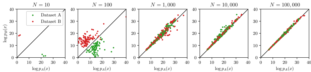
Figure 2: Convergence of energy estimates. The data set is split into two halves (denoted A and B), and separate energy models are trained on N samples drawn from each half. Each scatterplot compares the energy estimates of the two models at t = 0 , over all 2N training images. As N increases, the energy estimates of the two models converges for all images.
