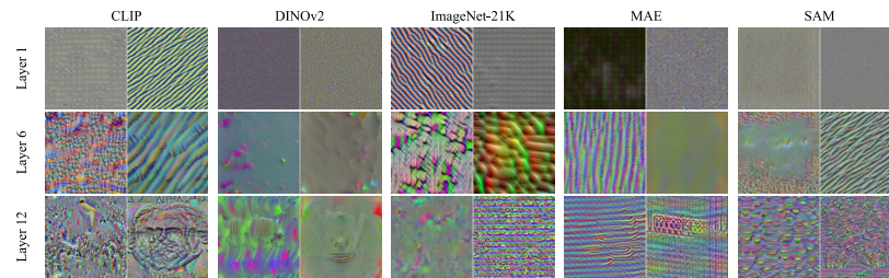
Figure 2: Images that maximise activations of different neurons of different models [1–3, 6, 7], using the technique from Ghiasi et al. [13]. All models rely on a ViT-B architecture, but each was trained with different data and supervision. Although all models usually pick up low-level patterns in early layers, distinct patterns appear as we get to intermediate and later layers, highlighting differences in learned representations. Models trained with ImageNet-21K, MAE, or SAM appear more sensitive to specific textures in later layers, whereas late CLIP neurons appear to react to patterns of semantic entities, and DINOv2 late neurons appear more sensitive to complex abstract shapes. These observations align with the idea that diverse features can be found by using multiple models, but also by using multiple layer outputs. Images are generated from randomly sampled neurons.
