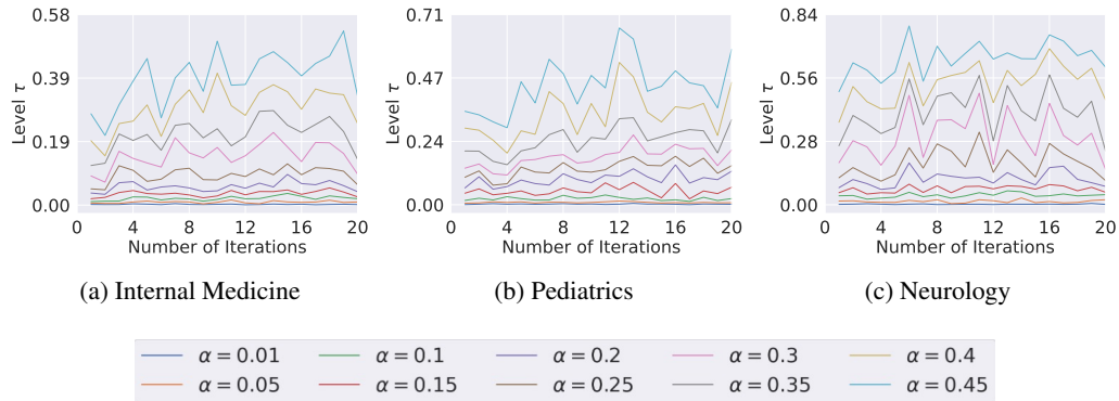
Figure 10: Thresholds obtained through split conformal prediction for MediQ. The legend below shows different colors. Each color corresponds to different choices of target coverage \alpha .
