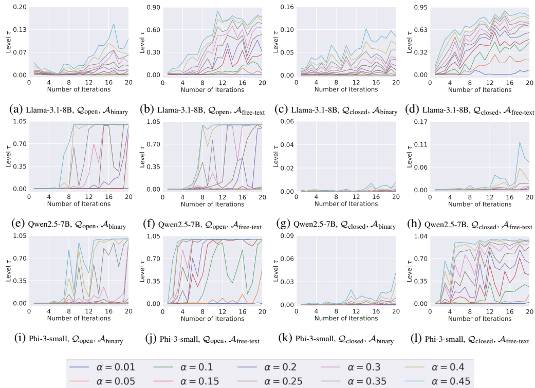
Figure 9: Thresholds obtained through split conformal prediction for 20Q. The legend below shows different colors. Each color corresponds to different choices of target coverage \alpha .
