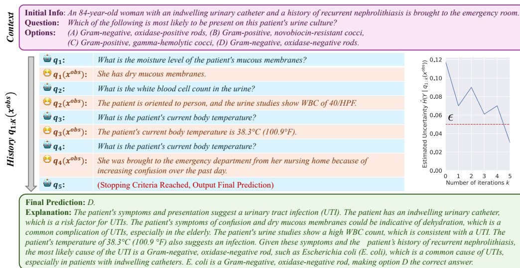
Figure 6: Example query-answer chain produced by C-IP for a patient in Internal Medicine. C-IP sequentially selects queries that approximately reduce uncertainty (i.e. average prediction set sizes from (11)) at each iteration. The posterior \hat{P}(Y | q_{1:k}(x^{obs})) is also estimated and a prediction is made. Once uncertainty drops below a chosen threshold \epsilon , the C-IP algorithm stops and makes a final prediction. Based on the obtained query-answer chain and the prediction, an explanation is also generated.
