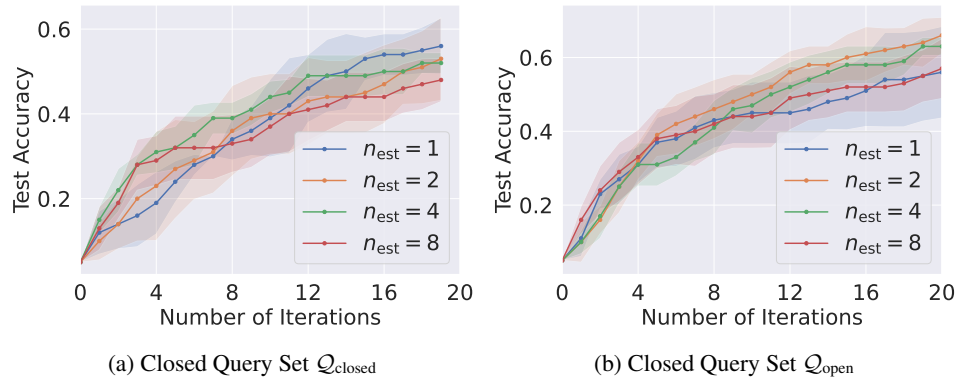
Figure 13: Performance of 20Q with different number of estimation samples. Each curve corresponds to the averaged accuracy over 5 runs, with shaded areas representing their standard deviation.
