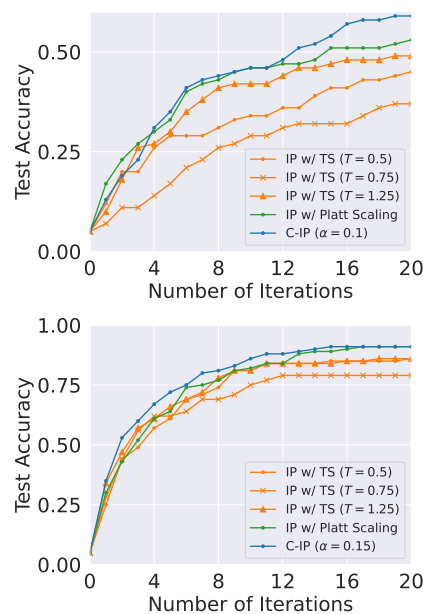
Figure 4: Comparison with Probability Calibration Baselines under open query set setting \mathcal{Q}_{\text{open}} with binary (top) and free-text (bottom) query answers.
