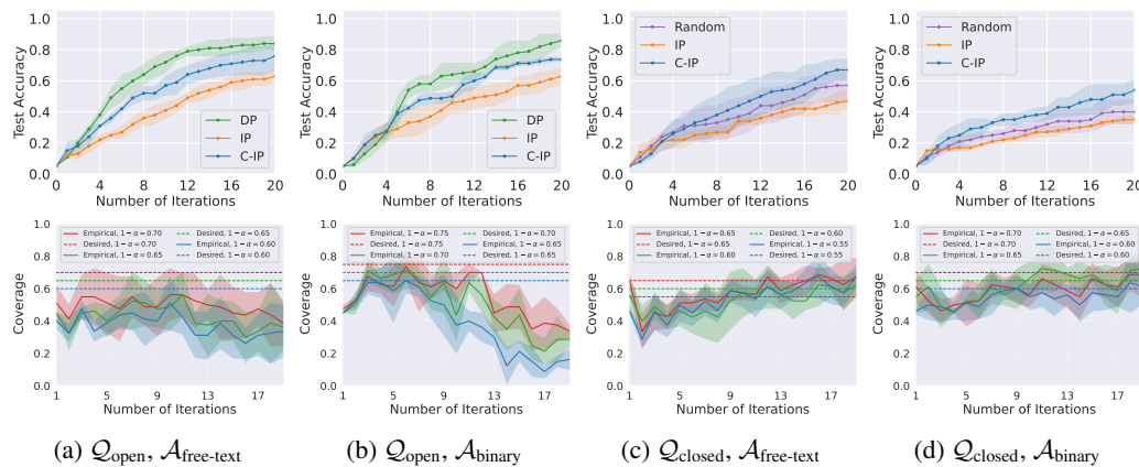
Figure 7: Predictive Performance of 20Q with Qwen-2.5-7B model.
