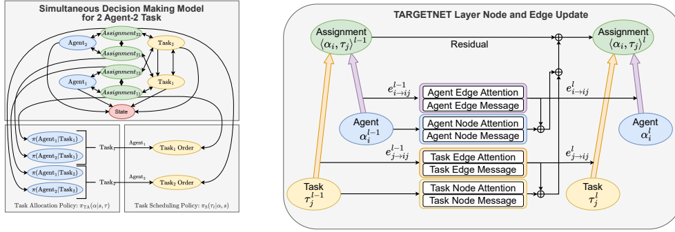
(a) Sample graph representation of a simple 2 agent-2 task problem, showing the heterogeneous nodes, and relationships for Task Allocation and Scheduling using TARGETNET.
