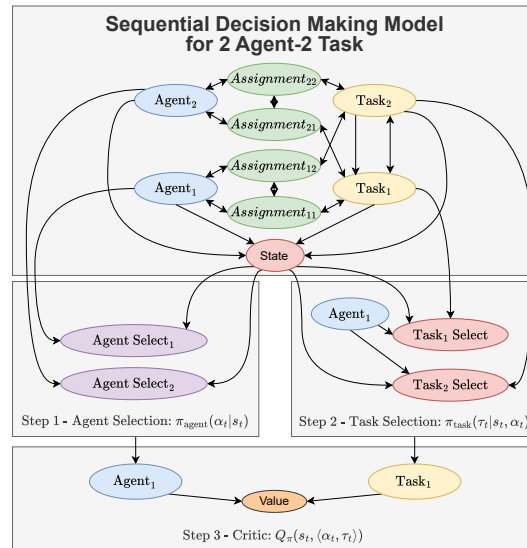
Figure 8: Sequential Decision Making for 2 Agent, 2 Task Problem, utilizing the relational environment representation to (1) select a agent, \alpha_t given state, s_t at step t , (2) select a task, \tau_t given state, s_t , and agent, \alpha_t at step t (3) evaluate the assignment of task, \tau_t , to agent, \alpha_t , for training using the Critic output, Q_t , at step t
