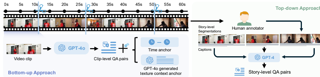
Figure 5: Overview of our video annotation framework combining bottom-up clip-level and top-down story-level approaches. The diagram illustrates our dual annotation strategy. In the bottom-up approach (left), short video clips are processed by GPT-4o to generate clip-level QA pairs enhanced with time anchors and textural context anchors. In the top-down approach (right), human annotators create story-level segmentations of longer videos, which are then captioned and processed by GPT-4 to generate comprehensive story-level QA pairs. This hierarchical methodology enables both fine-grained temporal understanding and high-level semantic comprehension of video content.
