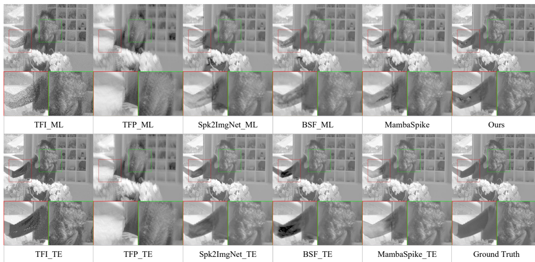
Figure 5: Visual comparisons of different reconstruction methods on the synthesized Kalantari13 dataset.
