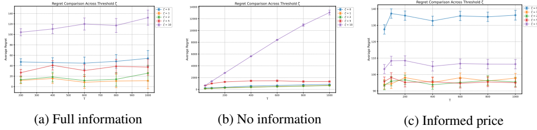
Figure 4: Regret of our algorithms under different thresholding parameters \zeta for (a) full information, (b) no information, and (c) informed price settings.
