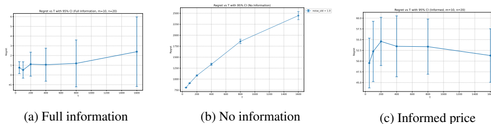
Figure 1: Regret of our algorithms under different time horizons T for (a) full information, (b) no information, and (c) informed price settings.
