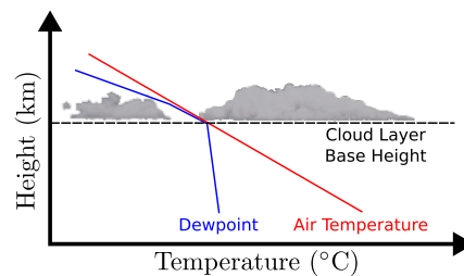
Figure 1: As a result of the cloud formation process, clouds are spatially structured into layers.
