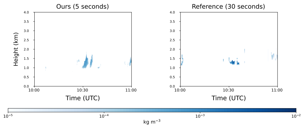
Figure 9: Example 1. Additional results comparing the liquid water content and liquid water path with radar retrievals.
