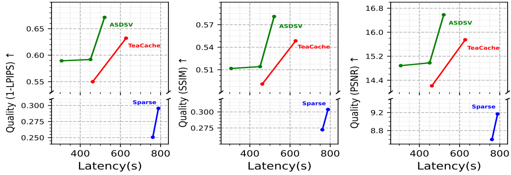
Figure 5: Quality-latency comparison of text-to-video diffusion models. The proposed ASDSV method demonstrates superior visual fidelity while maintaining lower inference latency compared to TeaCache[24] and Sparse VideoGen[38], evaluated under the Wan2.1 model.
