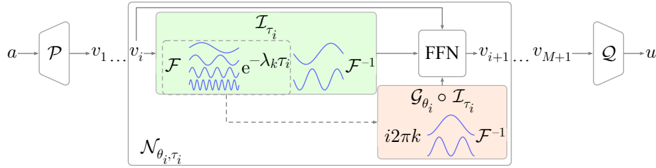
Figure 1: Overview of DINOZAUR. NO block \mathcal{N}_{\theta_i, \tau_i} is revised by updating the integral transform \mathcal{I}_{\tau_i} with diffusion multiplier \exp(-\lambda_k \tau_i) and including gradient features \mathcal{G}_{\theta_i} to add anisotropy. Feed-forward network (FFN) is applied to mix two sets of features.
