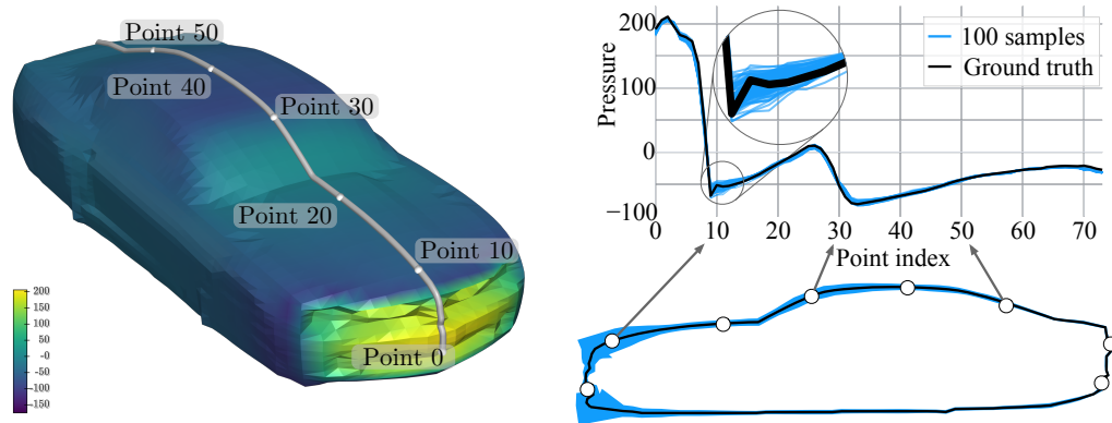
Figure 3: Uncertainty predictions. Left: mean of pressure samples on a test mesh with a geodesic path traced along the top. Right, top: ground truth and 100 sampled predictions along the same path. Right, bottom: car profile with a qualitative visualization of the standard deviation of pressure samples along the outline. High uncertainty is near sharp field changes, e.g., between Points 0 and 10.
